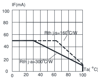
FIG.5 MAXIMUM FORWARD DC CURRENT VS AMBIENT TEMPERATURE ( T_{jmax}=110^{\circ}C )
