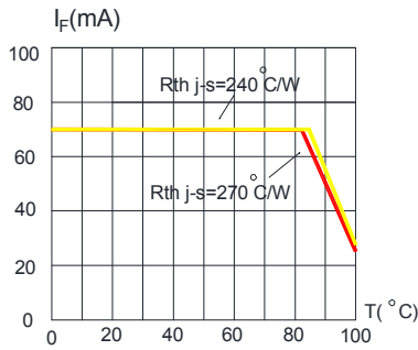
FIG.3 RED&AMBER MAXIMUM FORWARD DC CURRENT VS SOLDER TEMPERATURE (T jmax =110 °C)
